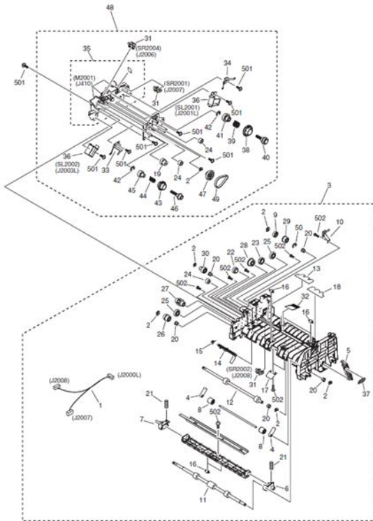
FIGURE 164A From SLX/SLY/SNK/SNL/SRS/SRT50001 PAPER FEED ASSEMBLY (NEW TYPE BELT DRIVE)
